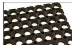
Supplier: Terram Product: Safety rubber matting 1x1.5m Thickness: 22mm Openings 250mm
