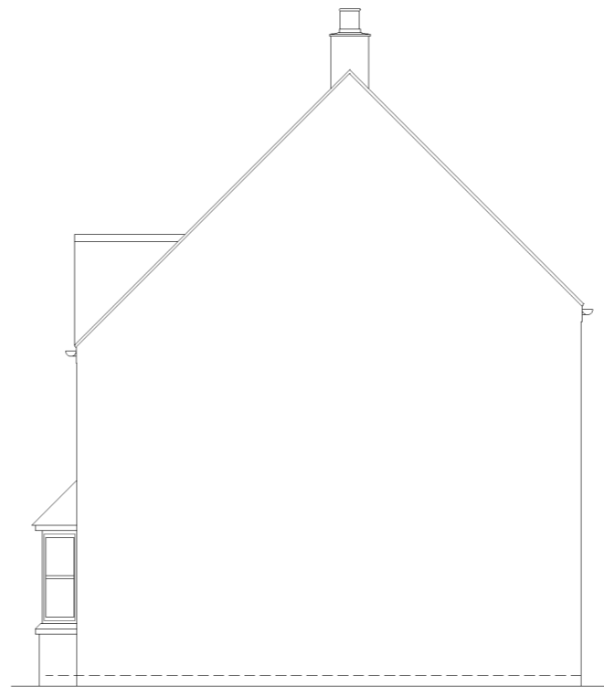
Side Elevation
