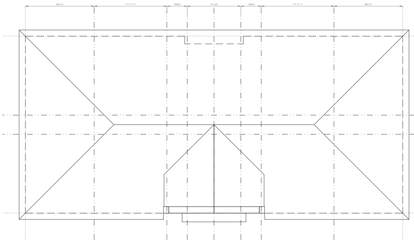
ROOF PLAN
