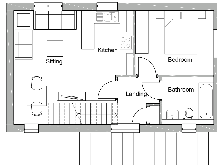
First Floor Plan Plot 20
