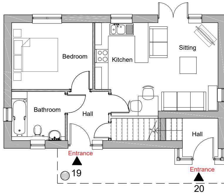
Ground Floor Plan Plot 19, 20
