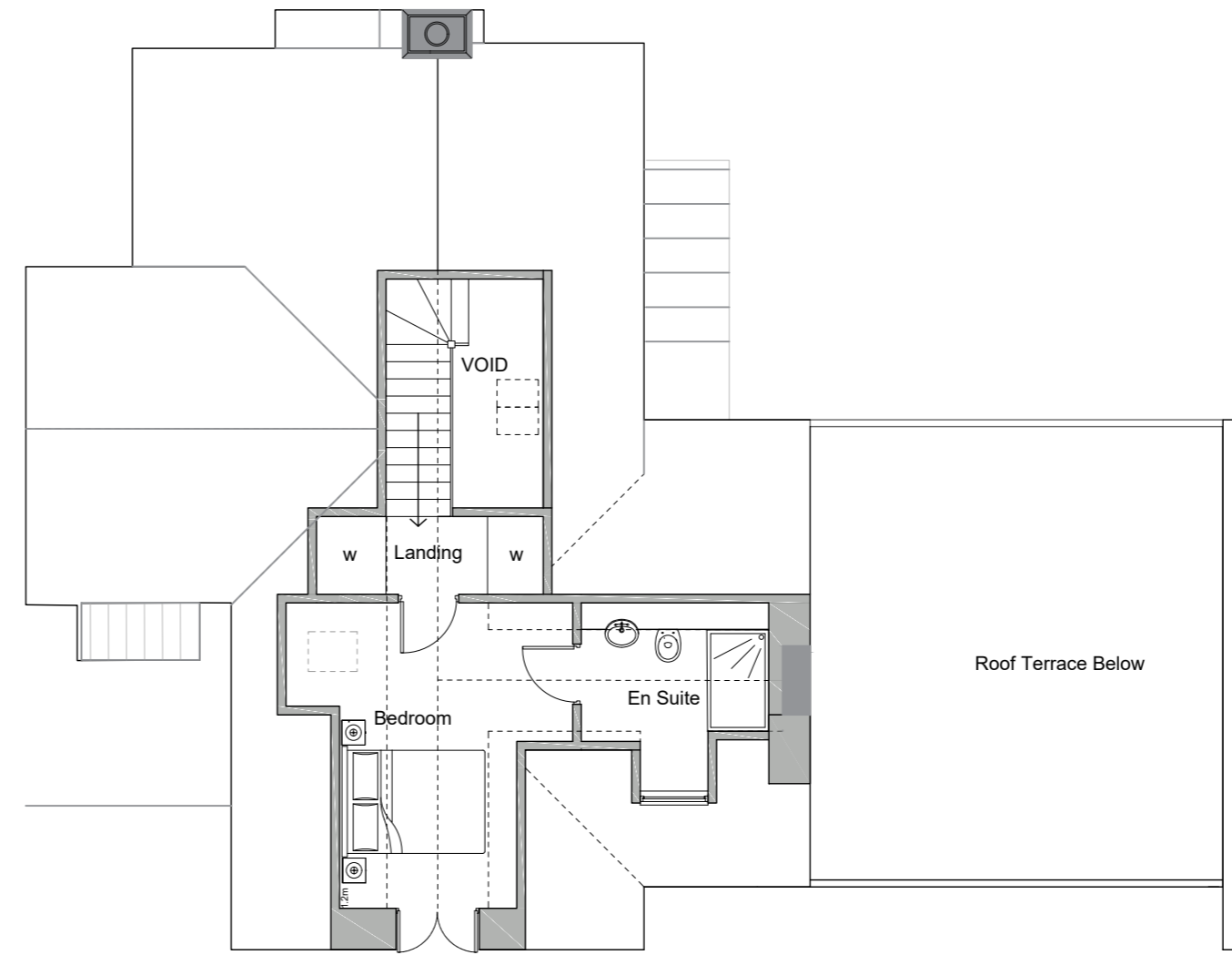
Attic Plan
