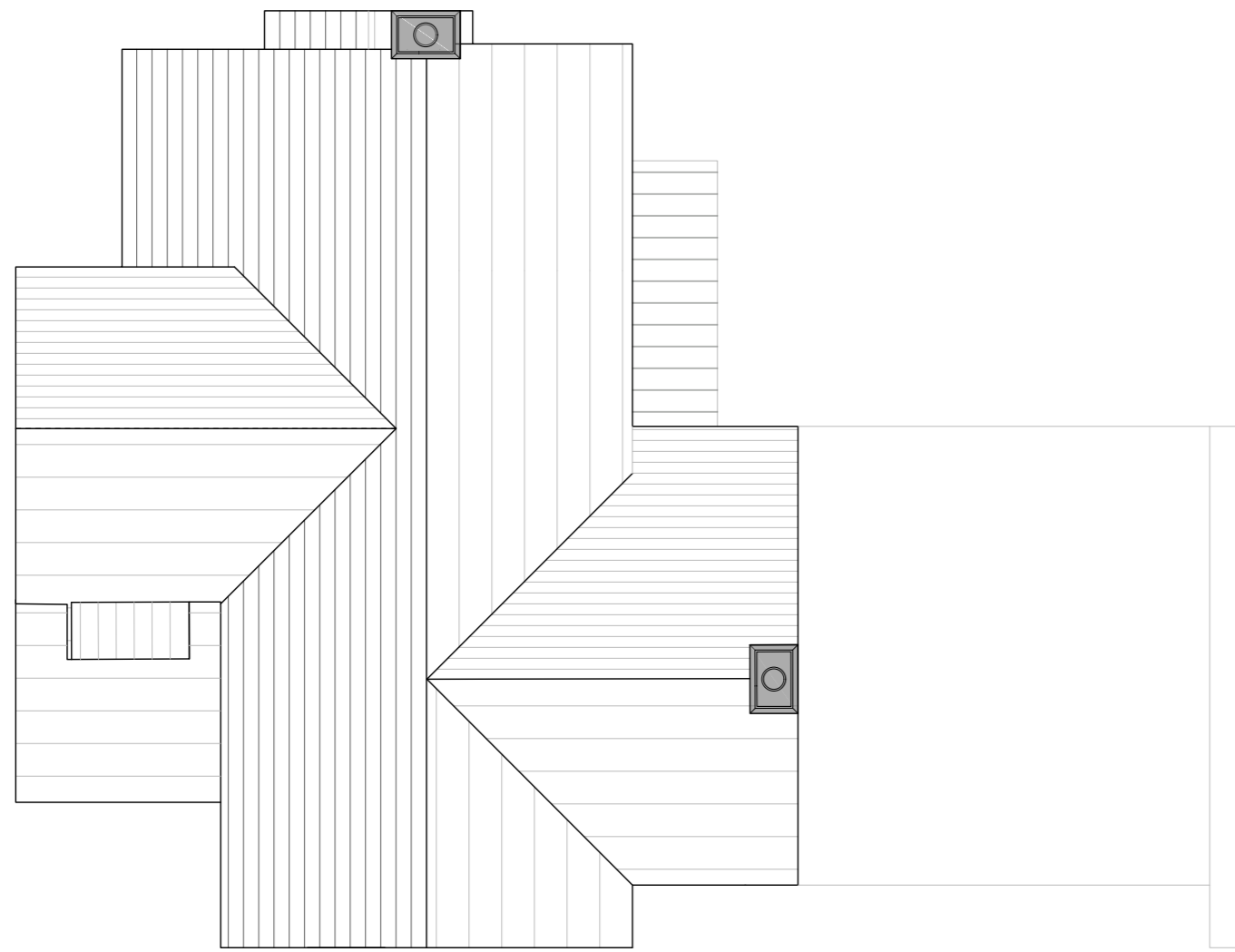
Roof Plan
