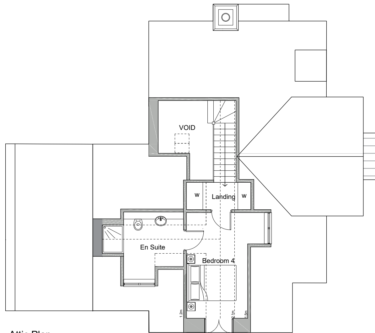
Attic Plan
