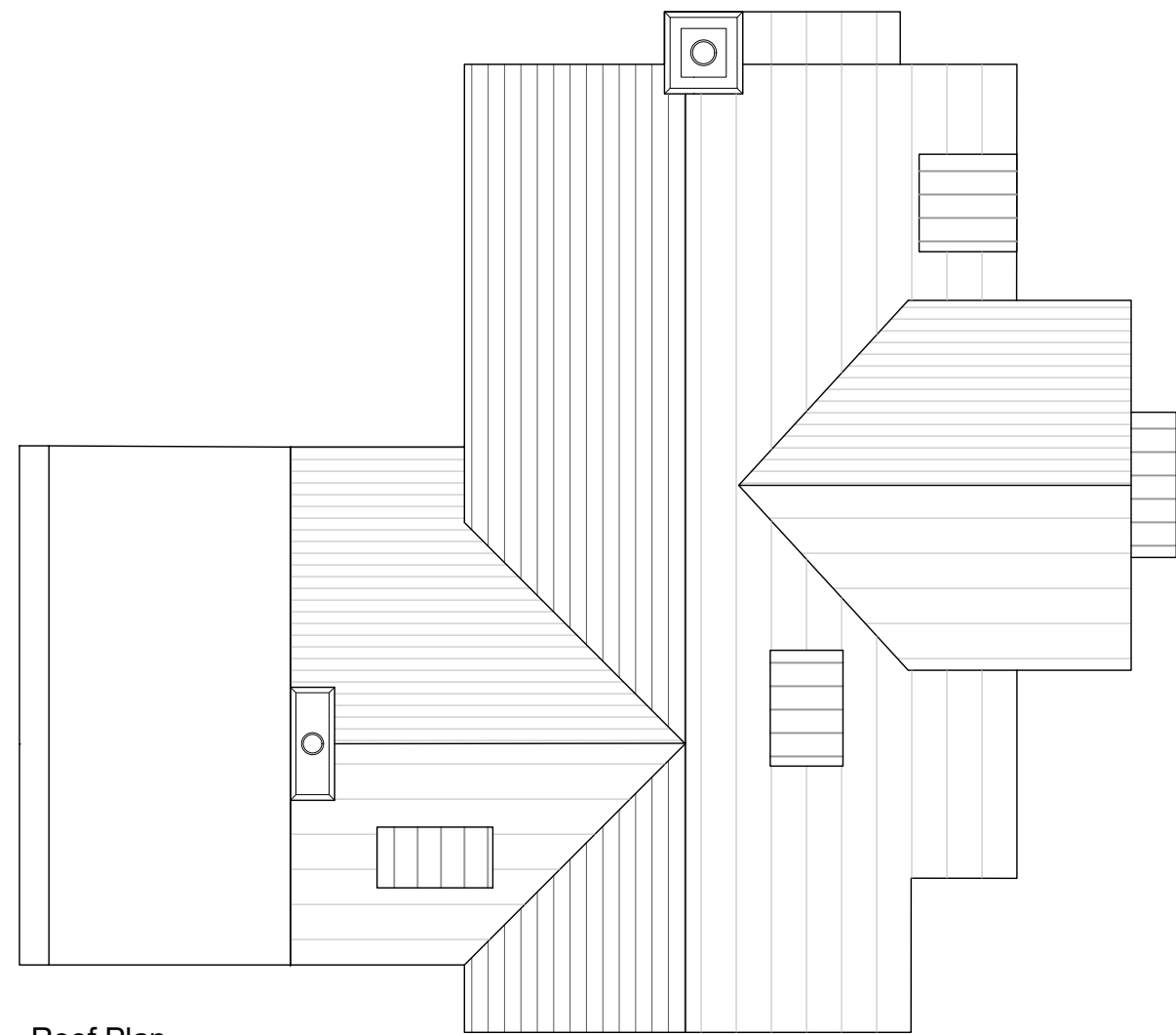
Roof Plan
