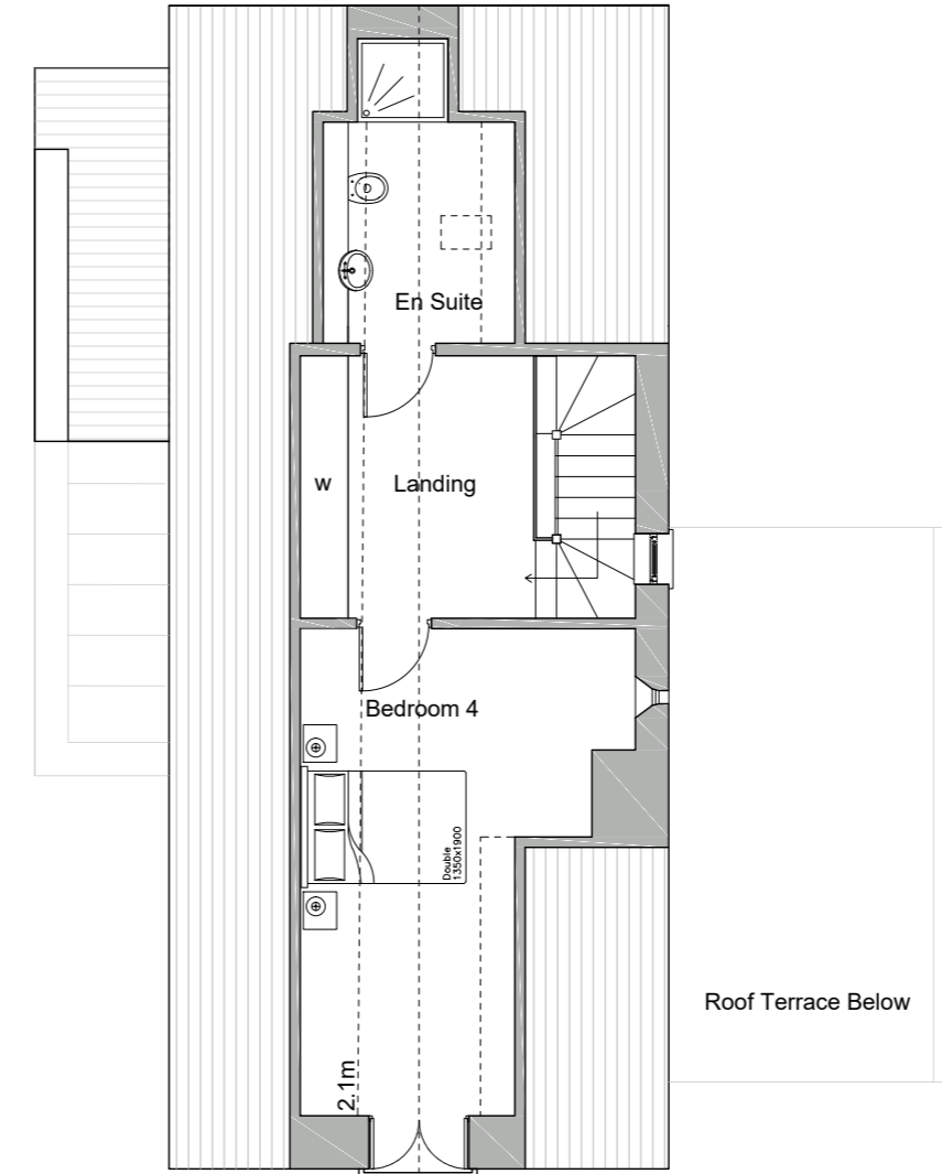
Attic Plan
