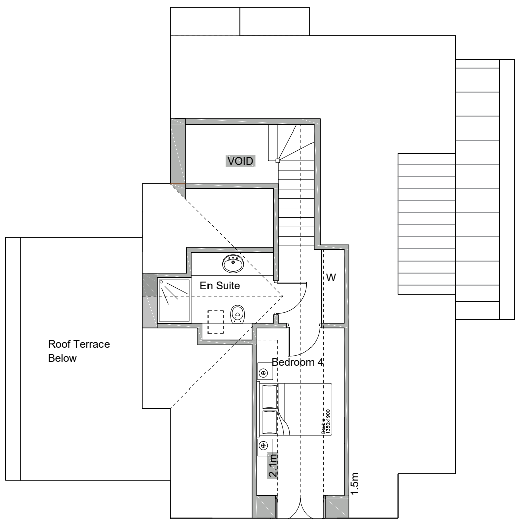
Attic Plan
