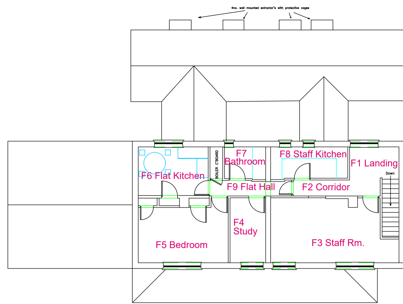
EXISTING FIRST FLOOR LAYOUT PLAN
