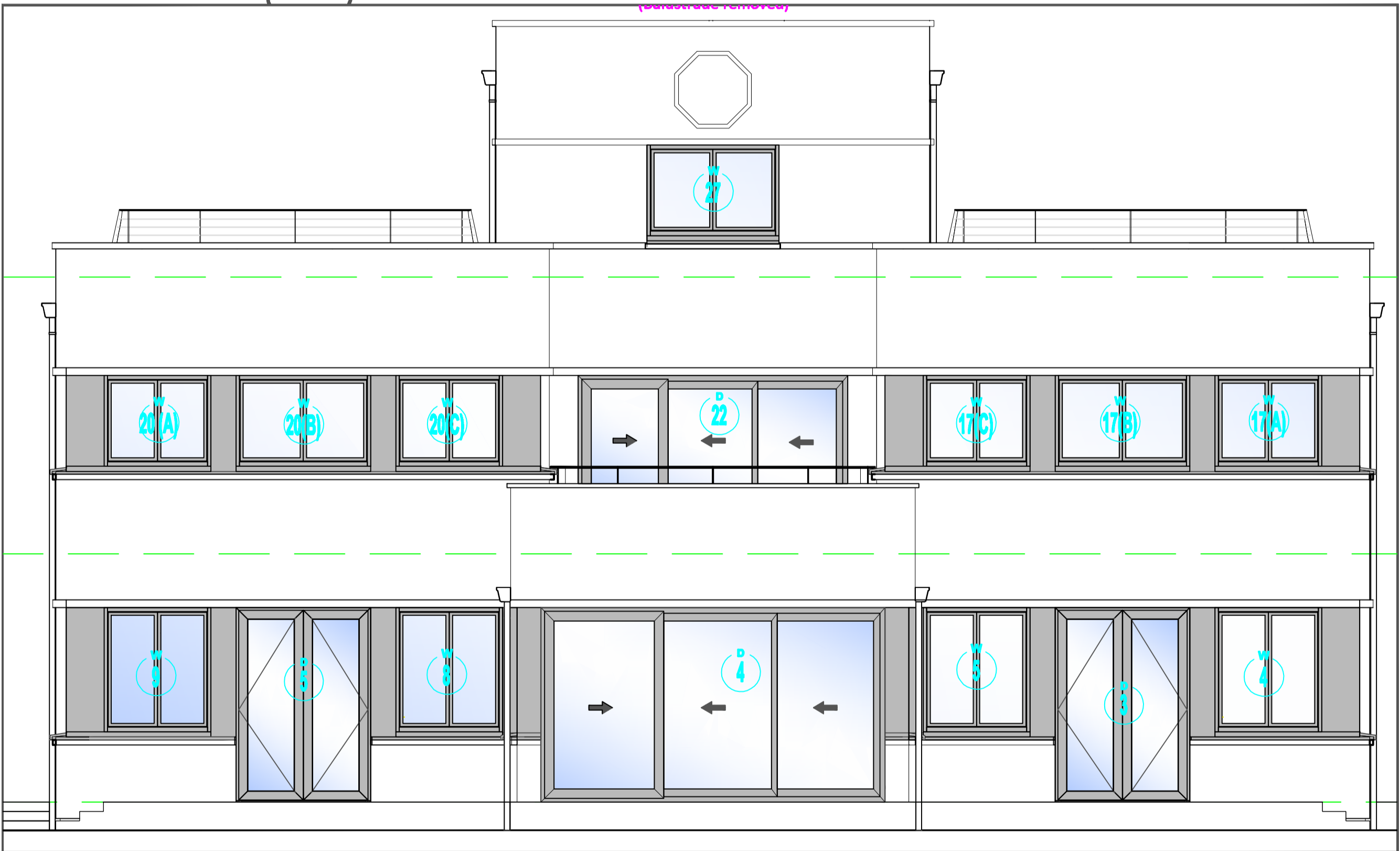
SIDE ELEVATION (WEST) 1:50
